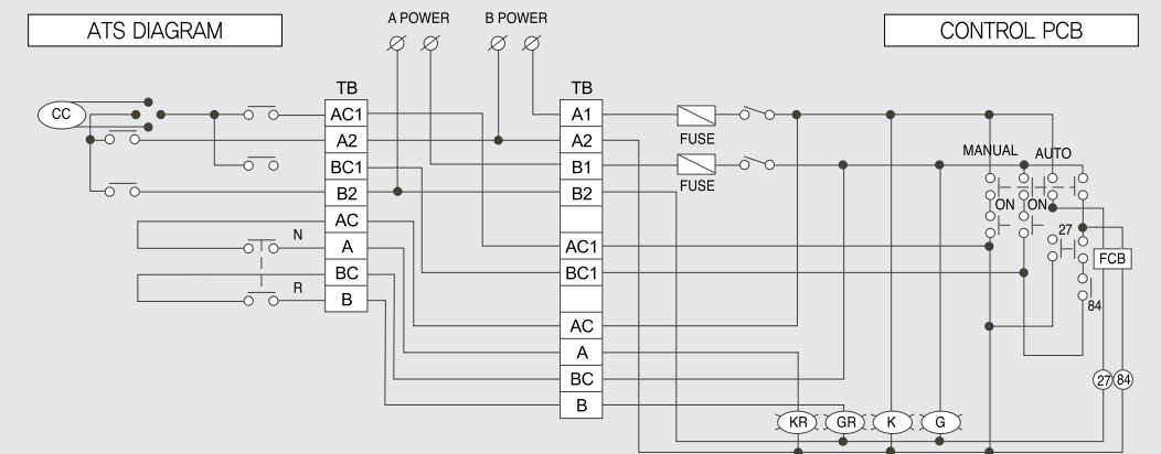
F Type ATS Control Sequence Diagram
