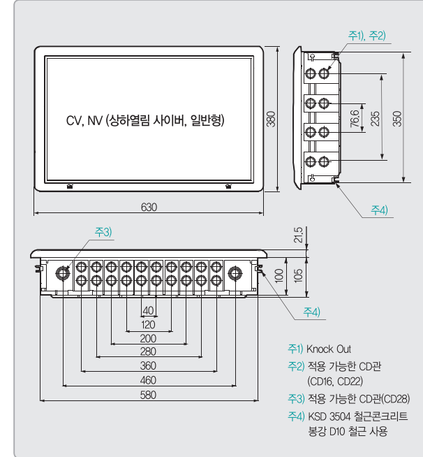
NV538 / NV638 / NV1038
