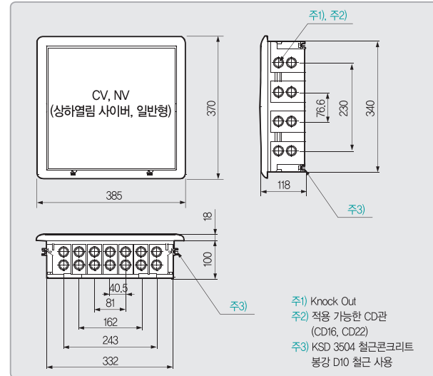
NV512 / NV612 / NV1012
